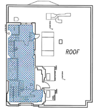
ROOF PLAN
